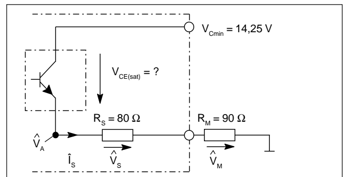
Fig. 8 Equivalent diagram for calculation of the available voltage V_A on the final stage of the amplifier.
