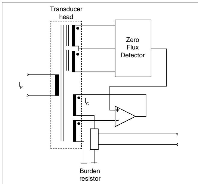
Figure 14 Total block diagram of closed loop IT transducers
