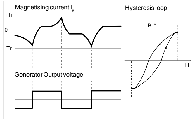
Fig. 13 Hysteresis loop and waveform signals
