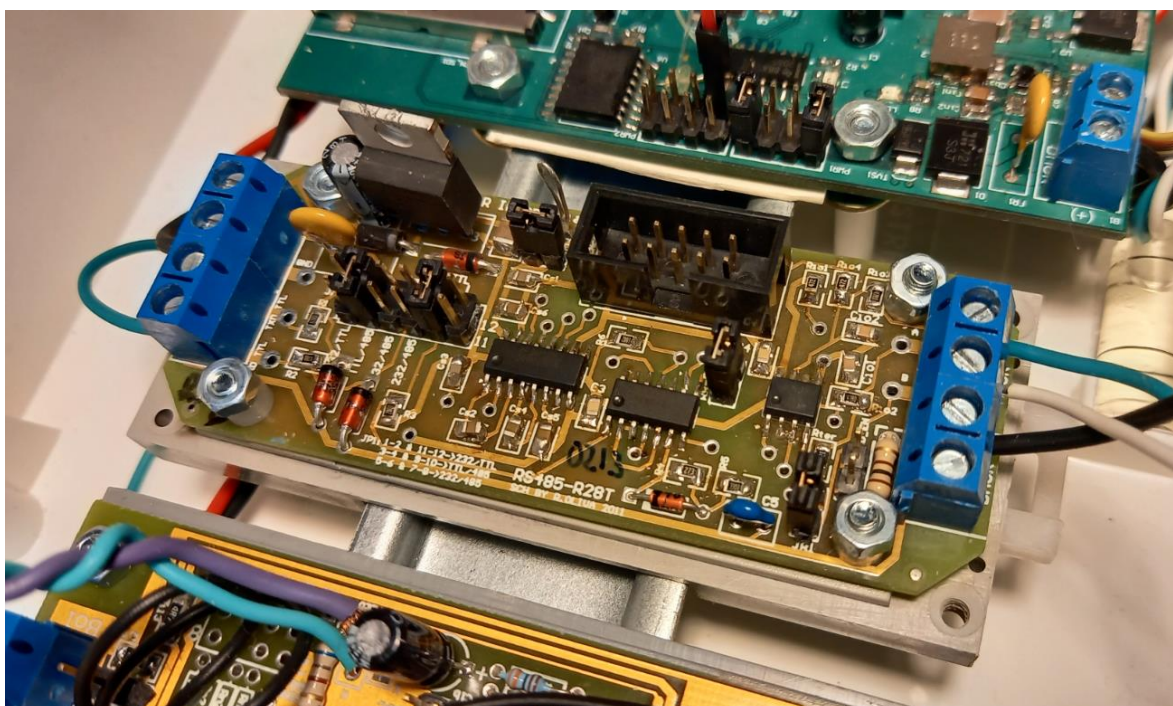
Figure 7b – Detail of hand-assembled DIN-RS485 board operating in TTL to RS485 Mode, connecting METEO to CL3
