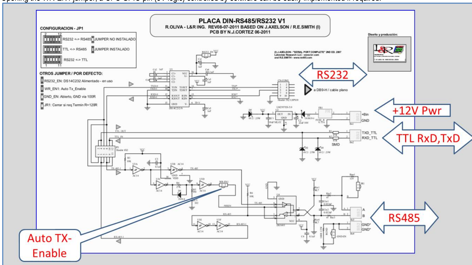
Figure 2 – Schematic and Functions of the DIN-RS485 board
