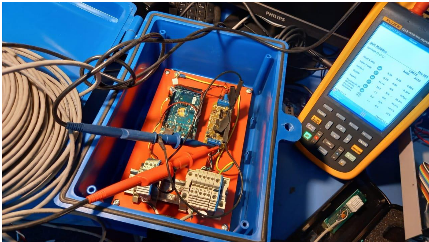
Figure 10 - The Modbus-RS485 bus health test was taken with a both probes connected to the differential A,B outputs referenced to GND, using UNPA's F125B Scopemeter
